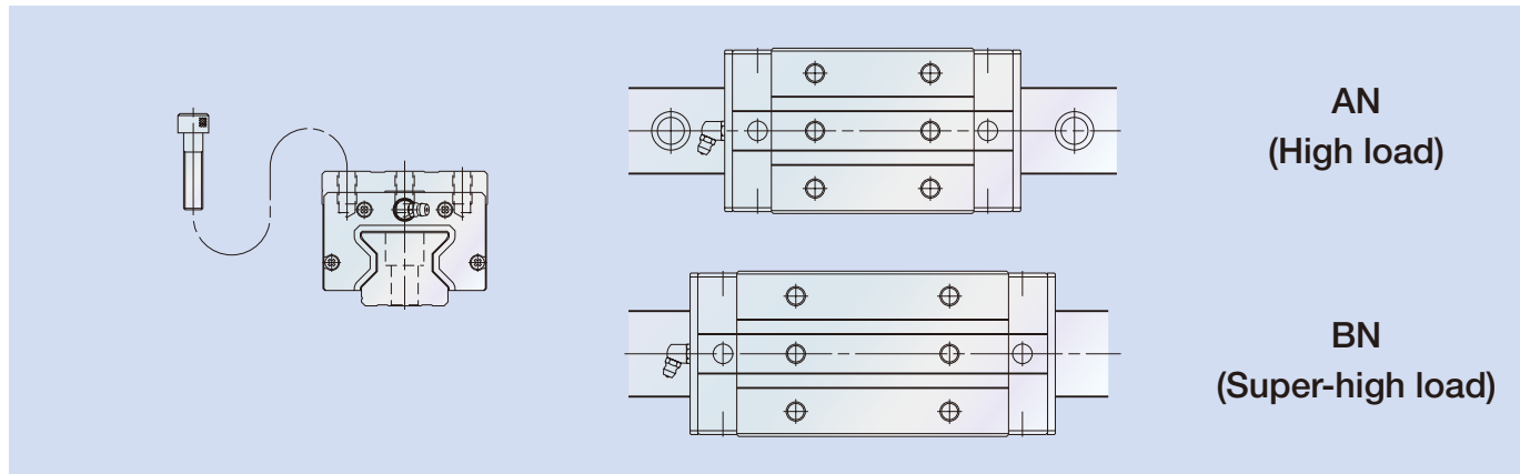
Fig. 1 Square type
