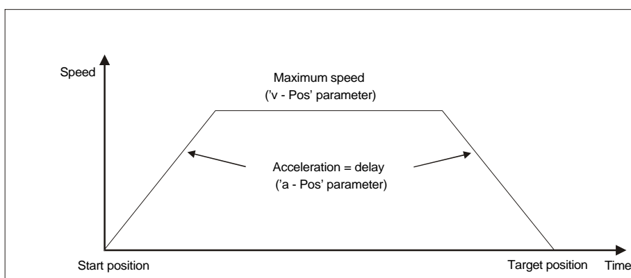
Fig. 2: Ramp travel in positioning mode (direct)
